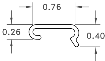
C Cleat (PVC)
