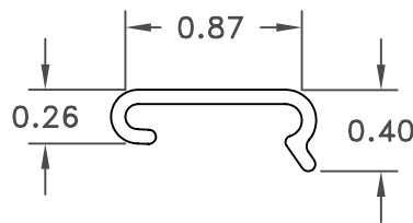
F Cleat (PVC)
