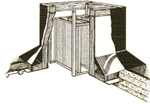
SOUND REDUCTION CURB*
