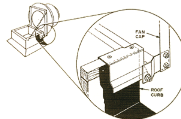
HINGE ASSEMBLY
