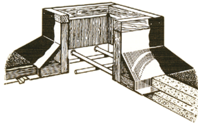
BURGLAR BAR CURB
