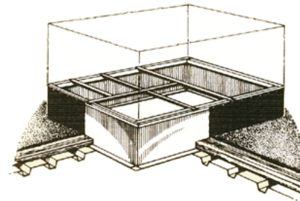
HVAC EQUIPMENT CURB
