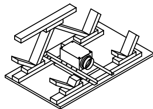
MODEL 55 DUCTED 90° THRU TRUSSES
