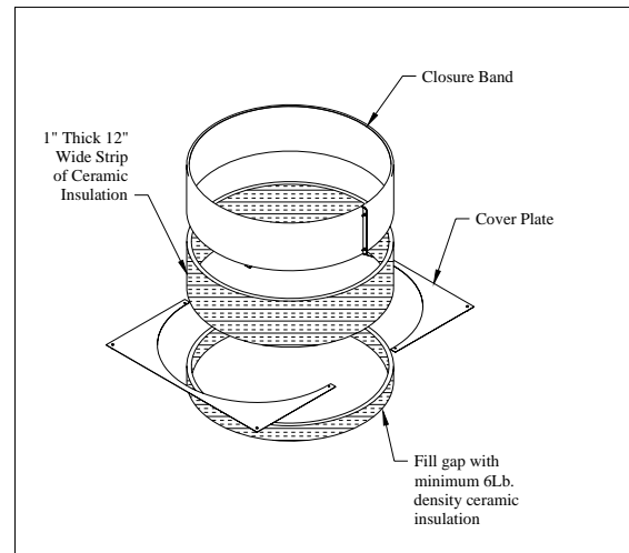
Fig. G-10 Isometric View of Through Penetration Firestop Kit
