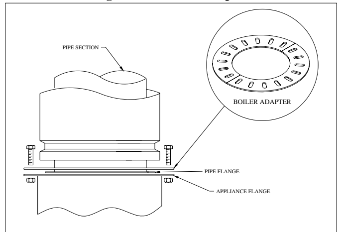
Fig. F-8 Boiler Kit Adapter
